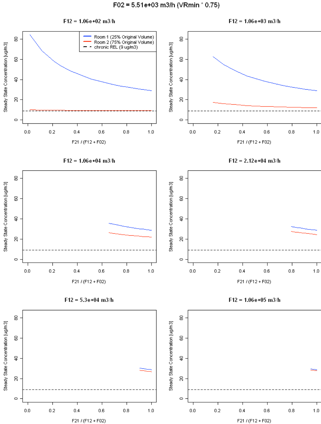
Figure 10. Scenario F – Steady state indoor air concentrations of formaldehyde in Zones 1 and 2, at specified F02 based on VRmin, and six values of F12, as F21 varies
