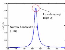
Figure 2: Typical power bode plot for resonant devices
