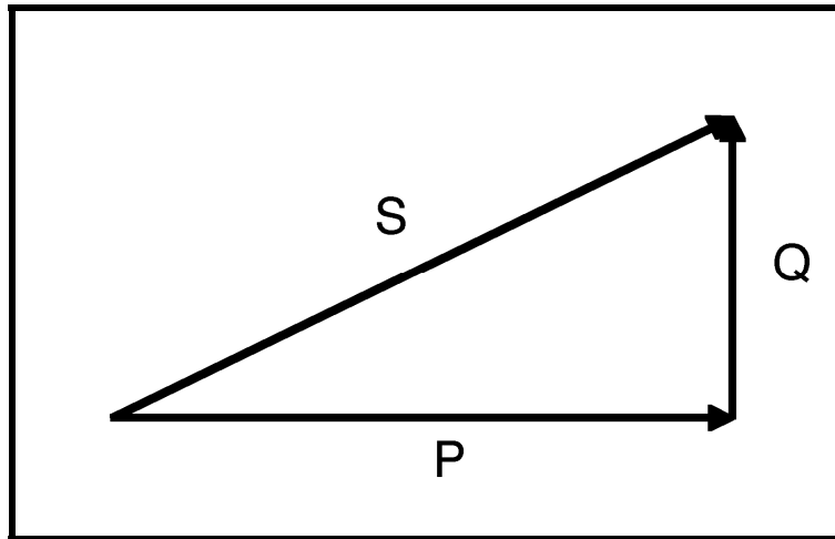
Figure 4. Relationship Between Power (P), Reactive Power (Q) and Total Power (S)
